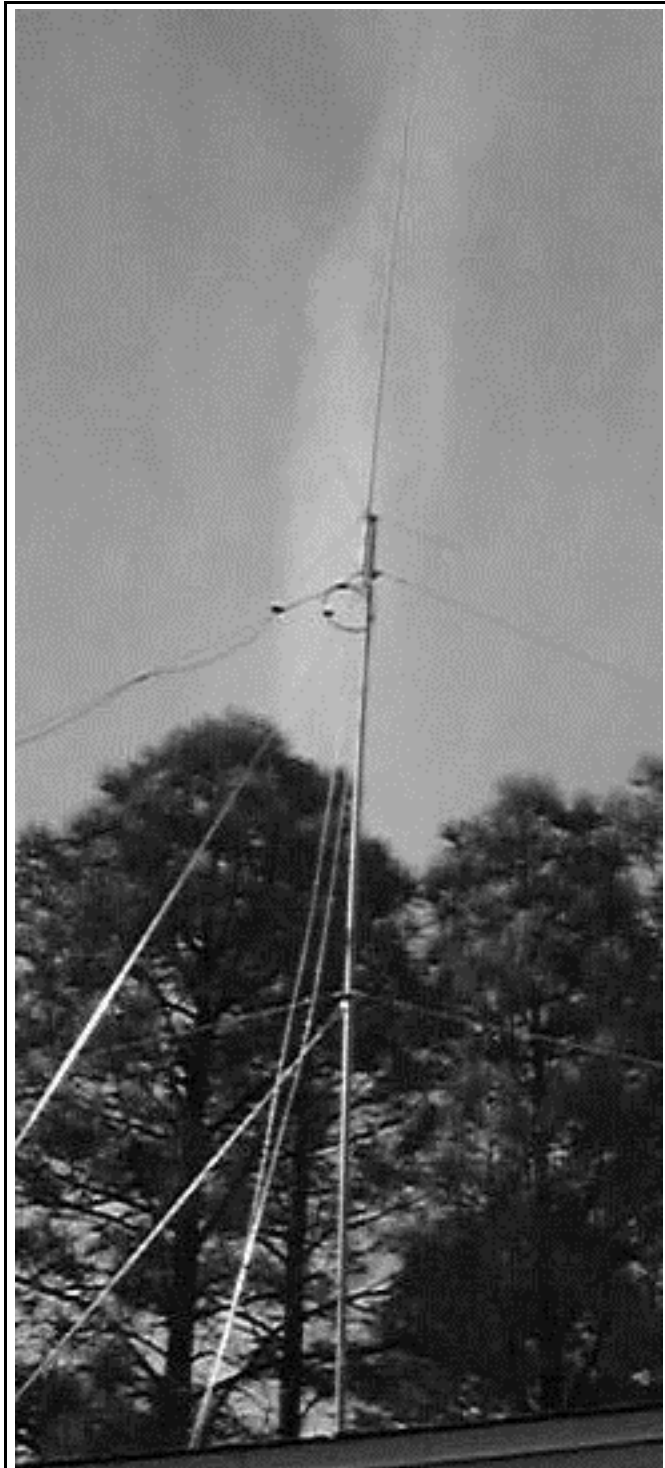
Picture 3: Ham Radio Antenna That I Raised View Showing the Guy Wires, January 24, 2006
